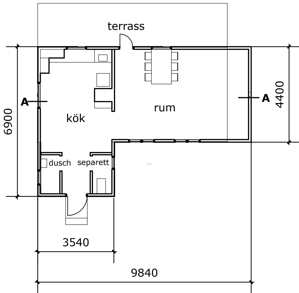
Plan
